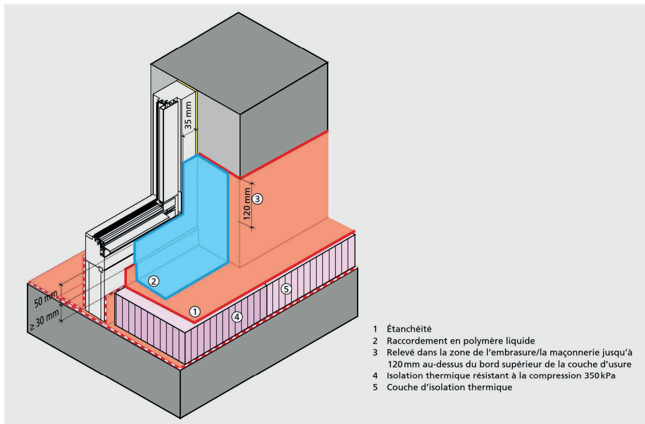
Figure 5.134: Raccordement d'embrasure au support.
